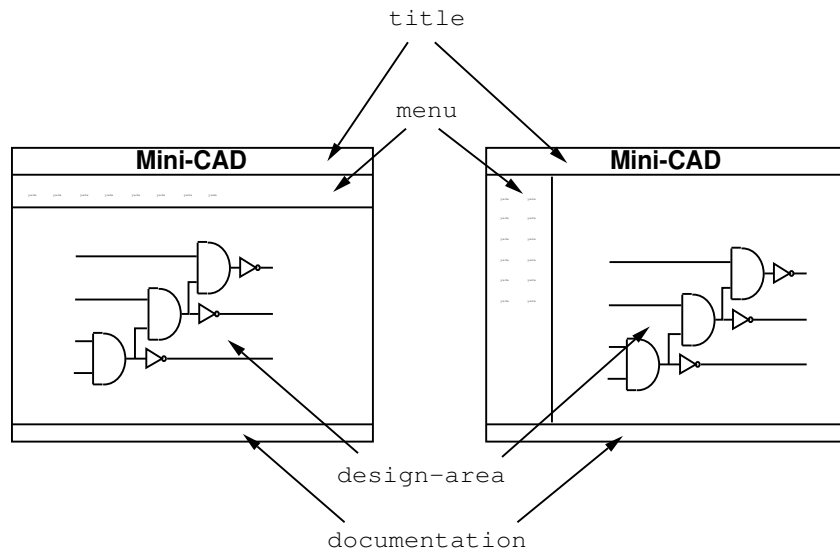
Figure 21. The two layouts of the Mini-CAD demo. Layout main is on the left, layout other is on the right.
