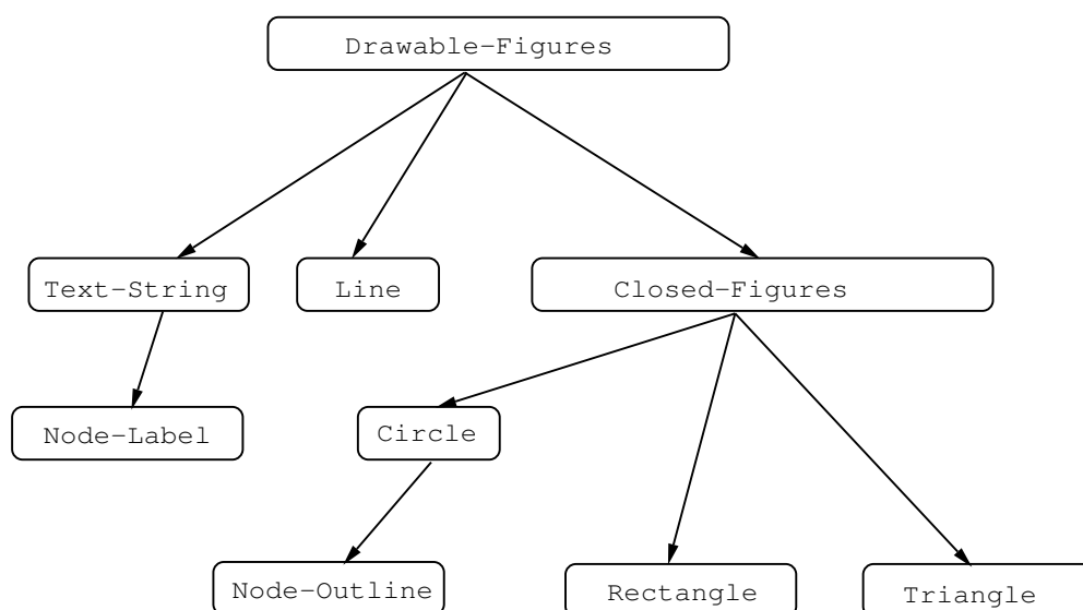
Figure 18. A collection of hierarchically related presentation types for a simple graphic editor
