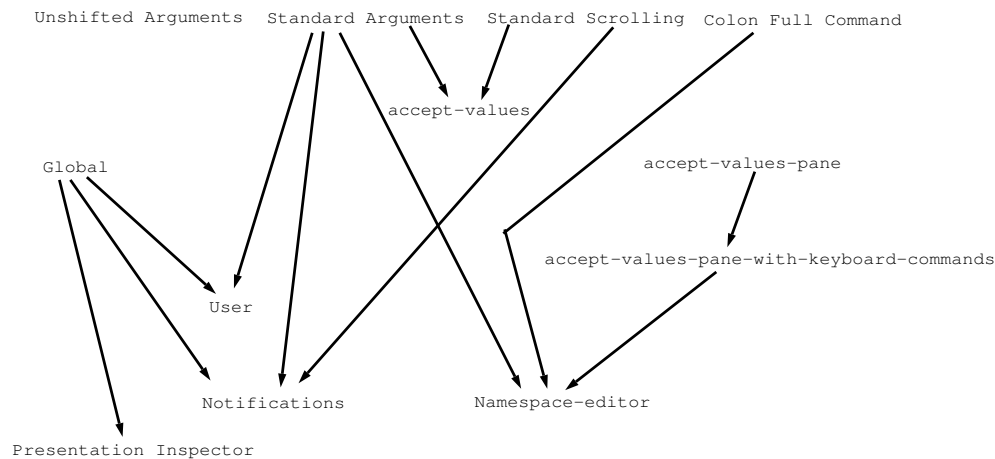
Figure 2. A sampling of system command tables
