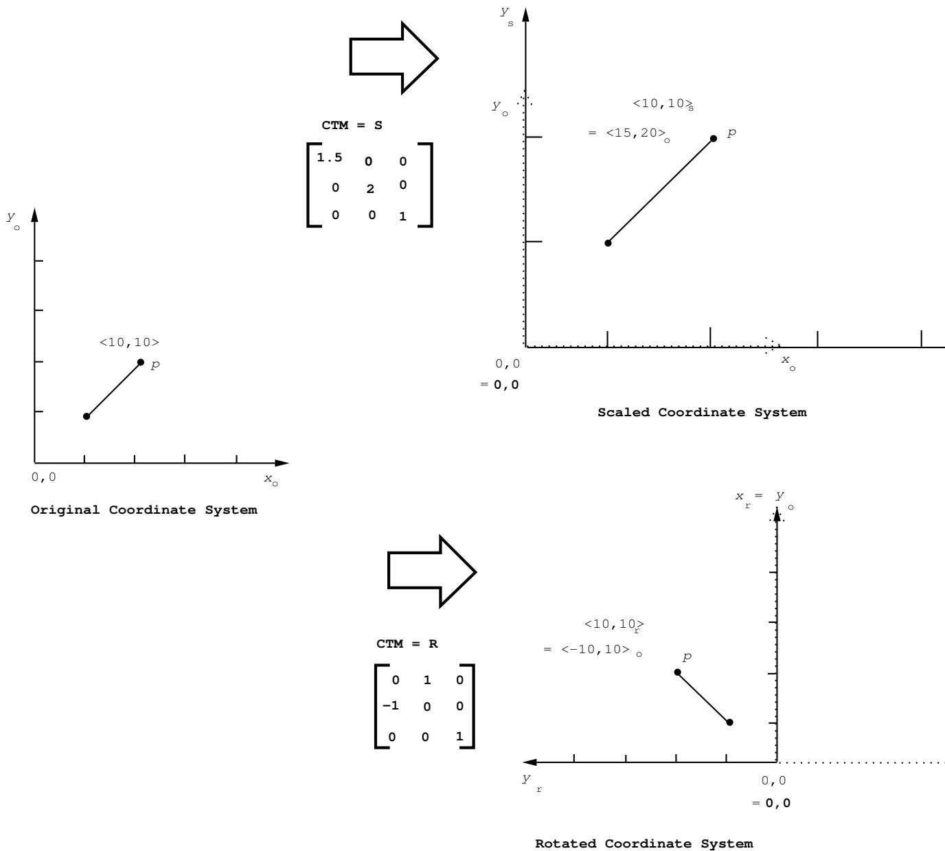
Figure 16. Changes effected by single coordinate transforms
