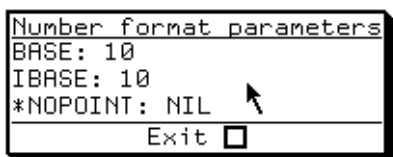
Figure 39. Choose-variable-values example 1.
